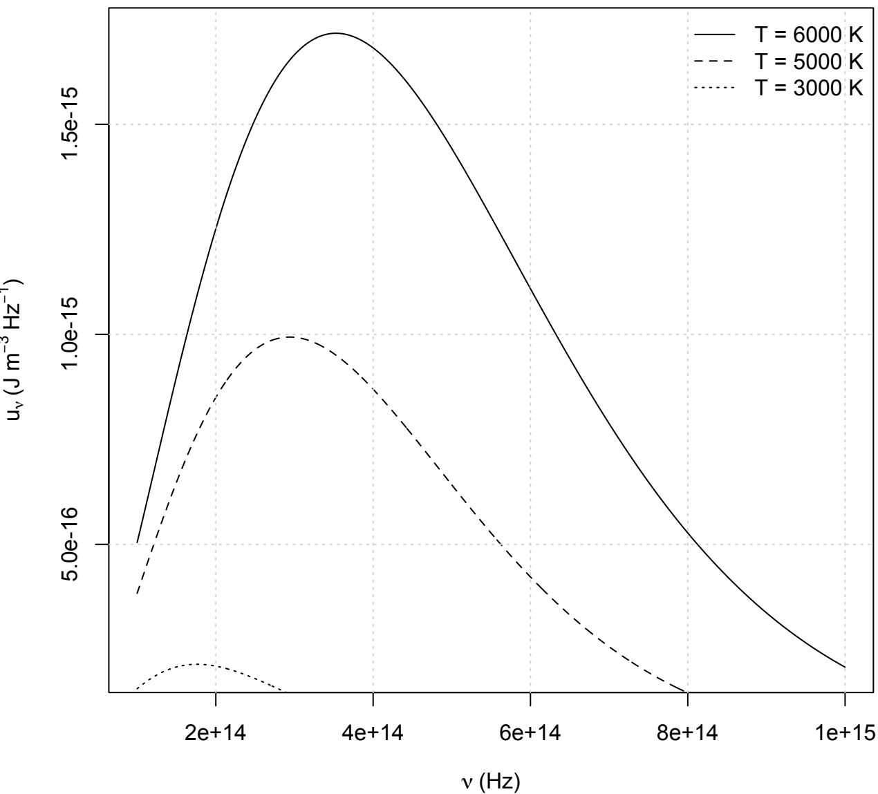
Planck spectral energy density u_\nu(\nu, T)
