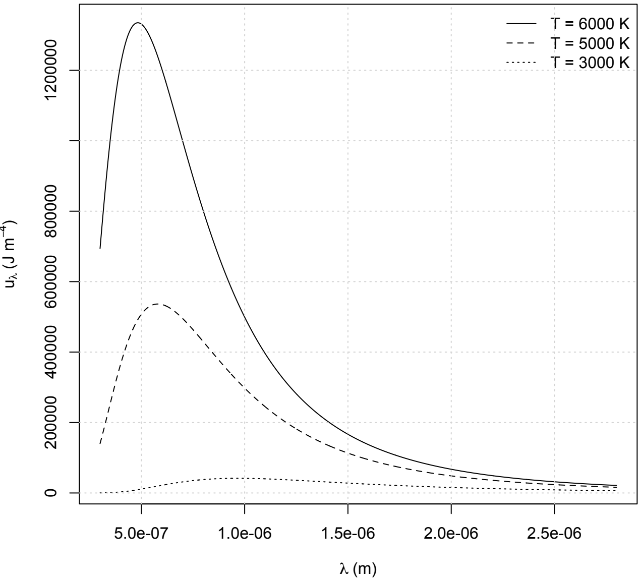
Planck spectral energy density u_\lambda(\lambda, T)
