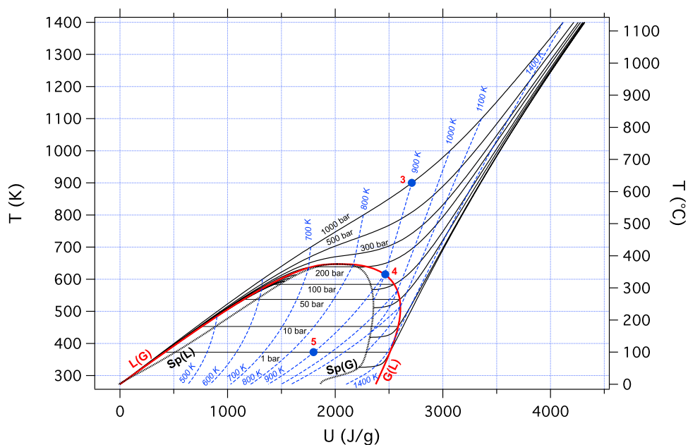
Figure 4. T - U diagram used for estimating the mechanical work produced by isentropic expansions. This diagram includes several types of curves: (1) isobars (full thin lines), calculated at 1, 10, 50, 100, 200, 300, 500, and 1000 bars; (2) isentropic decomposition curves (dashed lines) for a monophasic system; and (3) isentropic decomposition curves (dashed lines) for a biphasic system. Isentropic curves are labeled by their temperature at 1000 bar. Other elements of the diagram are the binodals (thick solid lines) L(G) and G(L) and the spinodals (dotted curves) Sp(L) and Sp(G) .
