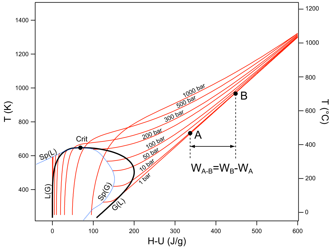
Figure 11. T - W diagram to calculate the work ( W = H - U , in J/g of water) produced by fluid isobaric expansion as a function of the initial and final temperatures. For example, to calculate the expansion work done by heating the fluid from point A ( T_A = 694 K) to point B ( T_B = 975 K) at constant pressure (here 1 bar), one makes the difference W_B - W_A ( = 450 - 320 = 130 J/g). Dotted lines are projections of the spinodal curves Sp(L) and Sp(G). Full thick lines are projections of the binodal curves L(G) and G(L). Thin solid lines are the isobars calculated at pressures of 1, 10, 50, 100, 200, 300, 500 and 1000 bars.
