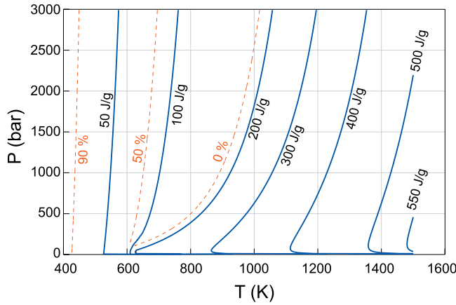
Figure 8. P - T diagram showing the mechanical work (full solid lines, in J/g of water) released by the irreversible adiabatic expansion of hot and pressurized steam as a function of the initial P - T conditions. Dashed lines indicate the liquid fraction (in mass percentage) of the gas-liquid mixture at a final state of 1 bar and 100°C. The field to the right of the 0% curve indicates the generation of superheated steams at 1 bar (i.e., with a final temperature above 100°C).
