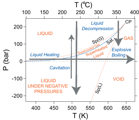
Figure 3. P - T diagram illustrating the different processes generating fluid instability. Solid line, saturation curve (Sat.); dotted lines, liquid spinodal curve Sp(L) and gas spinodal curve Sp(G) . These three curves meet at the critical point (CP).
