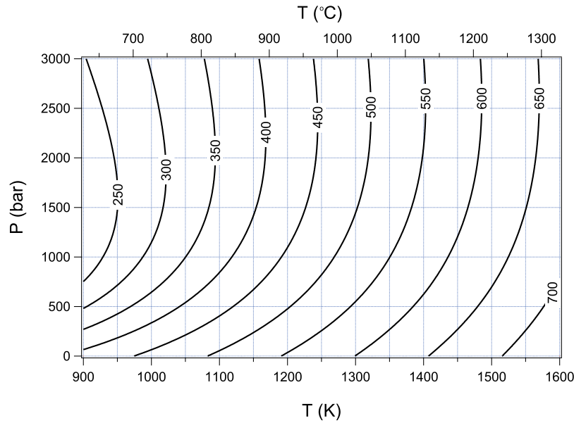
Figure 12. P - T diagram showing the work produced by the isobaric and isothermal exsolution of water from magma (in J/g of exsolved water) at fixed pressure P and temperature T .
