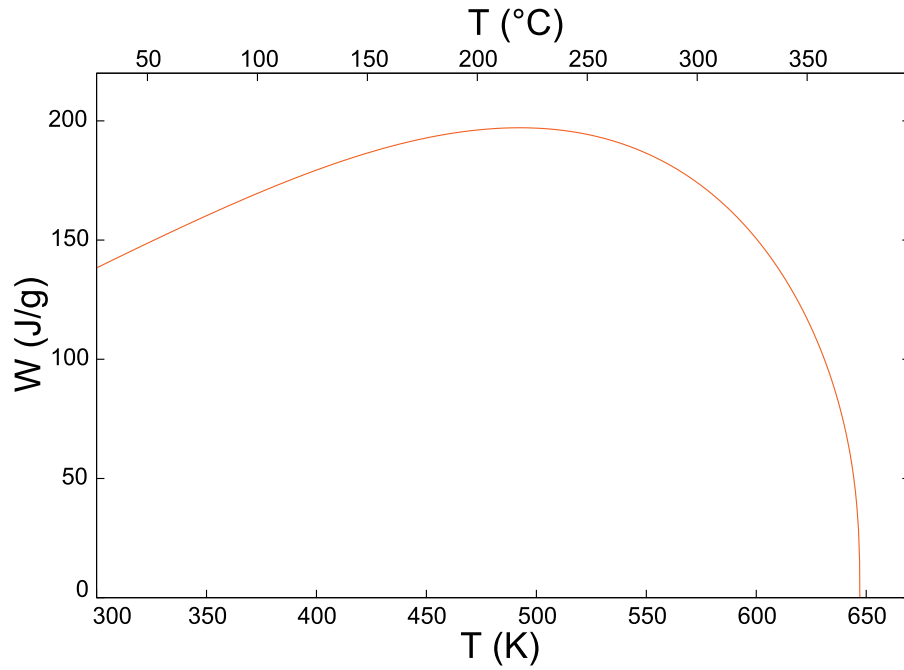
Figure 10. The mechanical work (in J/g of water) produced by liquid vaporization, as a function of the boiling temperature.
