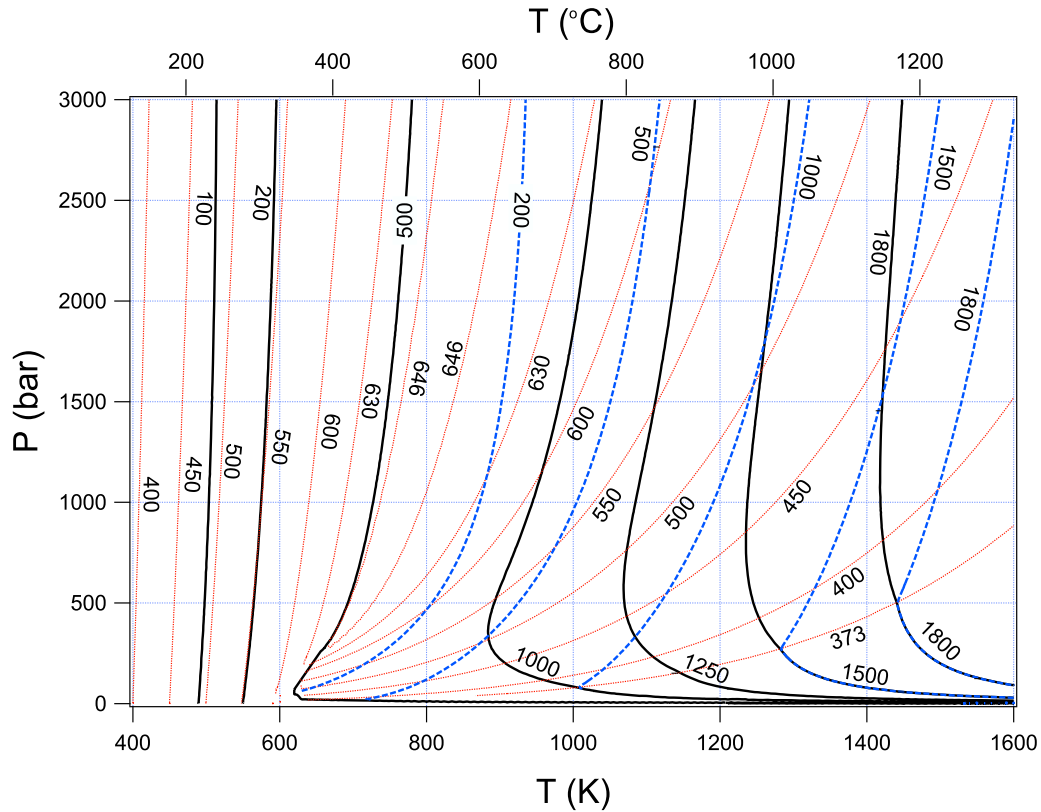
Figure 6. P - T diagram showing the mechanical energy released by the reversible isentropic expansion of hot steam (in J/g of water) as a function of the initial pressure P and temperature T in the magmatic chamber. Thick solid lines, total work ( W_U = U_5 - U_3 ) produced in the monophasic and biphasic fields; thick dashed lines, mechanical work ( W_{U,1} = U_4 - U_3 ) produced in the monophasic region; dotted lines, isotherms of the condensation temperature (in K) of the steam at 1 bar. Below the isotherm 373 K, both curves of monophasic and total works are coincident.
