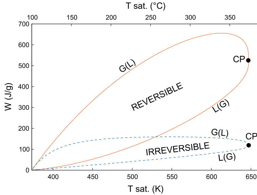
Figure 7. The expansion work (J/g of water) of a liquid-gas mixture against atmospheric pressure as a function of the initial saturation temperature. The full line indicates energies calculated for an isentropic decompression process, whereas the dashed curve is calculated for an irreversible adiabatic expansion. L(G), G(L), and CP represent, respectively, expansion works calculated for a saturated liquid, a saturated steam, and a critical fluid.
