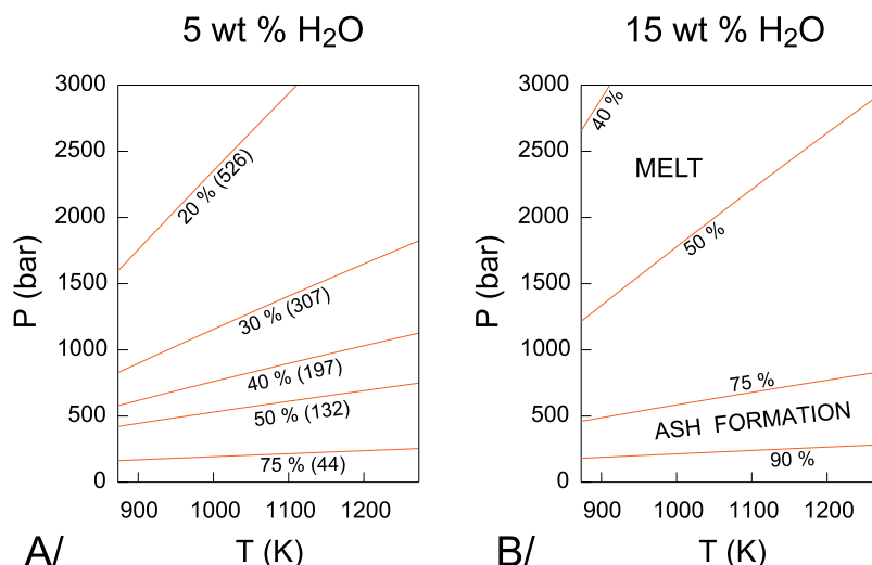
Figure 1. Water volume fraction ( f_v ) in a mixture of melt, crystals, and water as a function of the pressure P and temperature T , and for a water mass fraction of (a) 5% and (b) 15%. A value of 2500 kg/m 3 has been chosen for the density of the melt and solids. The density of water is calculated with the equation of state by Wagner and Pruss [2002]. Lines are iso- f_v curves. In Figure 1a, the corresponding density of the aqueous phase is indicated between parentheses in kg/m 3 .
