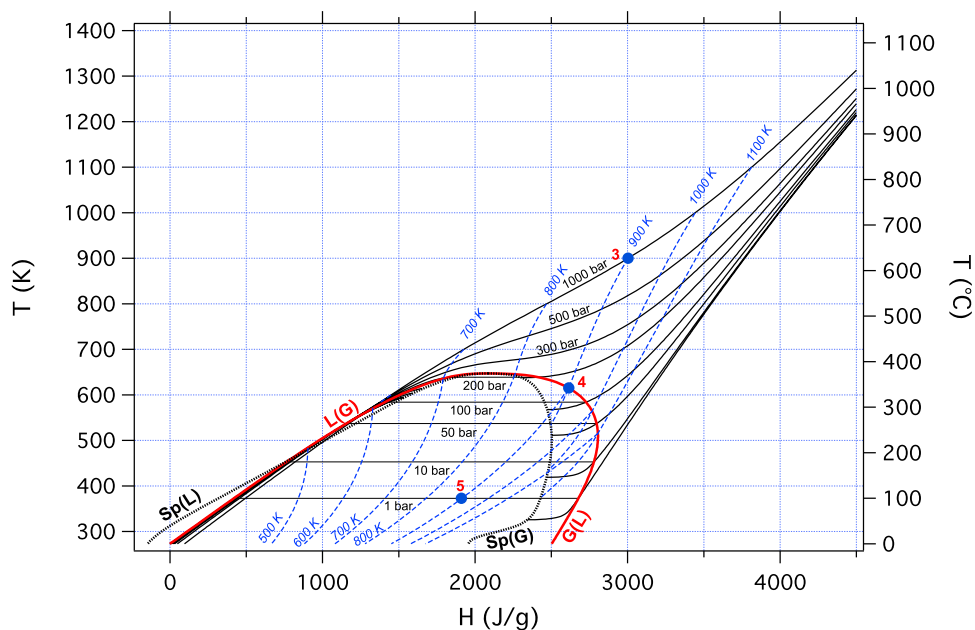
Figure 5. T - H diagram used for estimating isobaric heat transfer and mechanical work produced by isenthalpic or isentropic fluid circulations. This diagram includes several types of curves: (1) isobars (full thin lines), calculated at 1, 10, 50, 100, 200, 300, 500, and 1000 bars; (2) isentropic decomposition curves (dashed lines) for a monophasic system; and (3) isentropic decomposition curves (dashed lines) for a biphasic system. Isentropic curves are labeled by their temperature at 1000 bar. Other elements of the diagram are the binodals (thick solid lines) L(G) and G(L) and the spinodals (dotted curves) Sp(L) and Sp(G) .
