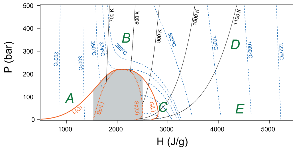
Figure 13. P - H diagram. Thick solid curves, binodal L(G) and G(L) curves; thick dotted curves, spinodal Sp(L) and Sp(G) curves; thin dashed curves, isotherms calculated at T = 200, 300, 350, 374 (critical isotherm), 390, 500, 750, 1000 , and 1227^\circ\text{C} ; thin solid lines, isentropic expansion curves labeled by the initial fluid temperatures at 1000 bars. Majuscule letters refer to as follows: A, liquid-dominated geothermal systems of low enthalpy; B, high-pressure hydrothermal systems of medium enthalpy; C, vapor-dominated geothermal systems of high enthalpy; D, exsolved magmatic, hot, and pressurized steams of vulcanian and plinian volcanic systems; E, hot and low-pressure steams produced by superficial phreato-magmatism. The shaded area indicates explosive liquid-gas demixing conditions.
