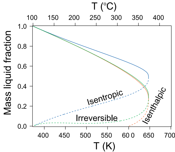
Figure 9. The mass liquid fraction of the liquid-gas mixture at 100°C and 1 bar produced by the depressurization of a saturated liquid (full curve) or saturated steam (dashed curve), as calculated by three types of decompression processes, i.e., isentropic, isenthalpic, and irreversible expansions.
