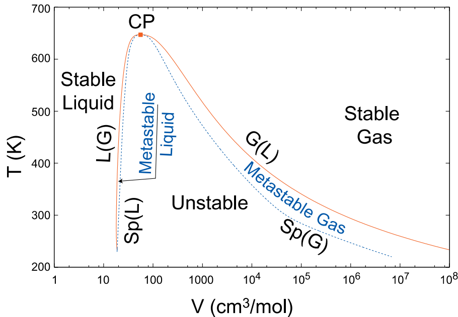
Figure 2. The stable, metastable, and unstable fields of water projected in the T - v space. The full lines separating the stable and metastable regions are the binodal curves; the first branch, noted L(G), refers to the saturated liquid water, whereas the other one, noted G(L), refers to the saturated steam. Both branches join at the critical point (noted CP). The dashed curves are the two spinodal curves, which start from the critical point and delimit the unstable field from the metastable region. The first one, noted Sp(L), is the liquid spinodal curve, and the second one, noted Sp(G), is the gas spinodal curve.
