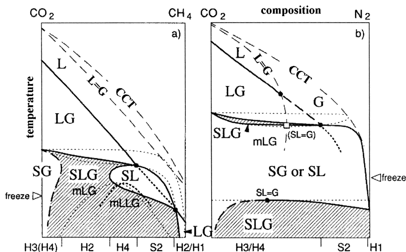
Fig. 6. Topology of isochoric TX diagrams (molar volume \sim 50 \text{ cm}^3/\text{mole} ) for the systems \text{CO}_2\text{--CH}_4 and \text{CO}_2\text{--N}_2 . Shaded area shows the stability of coexisting SLG. L = G is the (polychoric) critical curve; CCT is the 'cricondentherm', the maximum extension of the LG-immiscibility (see text for explanation).
