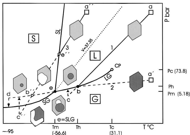
Fig. 2. Schematic PT diagram showing phase transitions for inclusions trapped at a , a' , and a'' (see text for explanation). Fillings in the fluid inclusion icons: dark gray = gas phase; light gray = liquid; white = solid phase.
