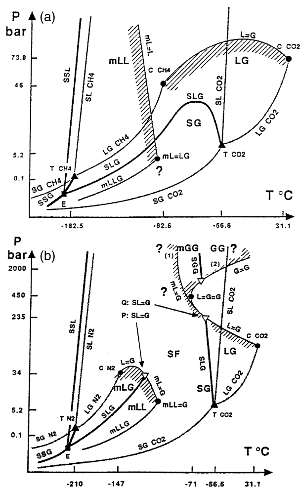
Fig. 5. Topology of the systems CO 2 -CH 4 (a) and CO 2 -N 2 (b), after Thiéry et al. (1994b). The pressure and temperature scales are arbitrary. Invariant points: eutectic point (E, filled square), triple points (T, filled triangles), L = G CPs for pure fluids (C, filled circles), three-phase critical end-points (filled circles), SL = G intersection points of a critical curve with the SLG curve (triangles). Univariant lines: two-phase assemblage for the pure end-members (gray lines), three-phase assemblage for the binary systems (thick solid lines), and critical curves (thin solid lines). The prefix 'm' denotes metastable parts. Regions around the triple points T_{CH_4} and T_{N_2} are enlarged. The critical curves (L = L and L = G) delimit LL and LG immiscibility (shaded areas). Also indicated are the stability fields of liquid-liquid (LL), solid-gas (SG) and solid-fluid (SF). The calculated extensions of the critical curve towards high pressures for CO 2 -N 2 are sketched according to (1) Thiéry et al. (1994b) and (2) Kreglewski and Hall (1983). The pressure and temperature scales are arbitrary.
