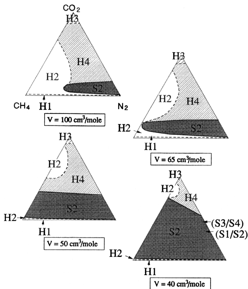
Fig. 13. Isochoric projections of the system \text{CO}_2\text{--CH}_4\text{--N}_2 showing the behavior on microthermometry runs in relation to composition and molar volume. Diagrams are shown for 40, 50, 65 and 100\text{ cm}^3/\text{mole} . Note that T_h < T_m for the dark gray areas denoted by S2.
