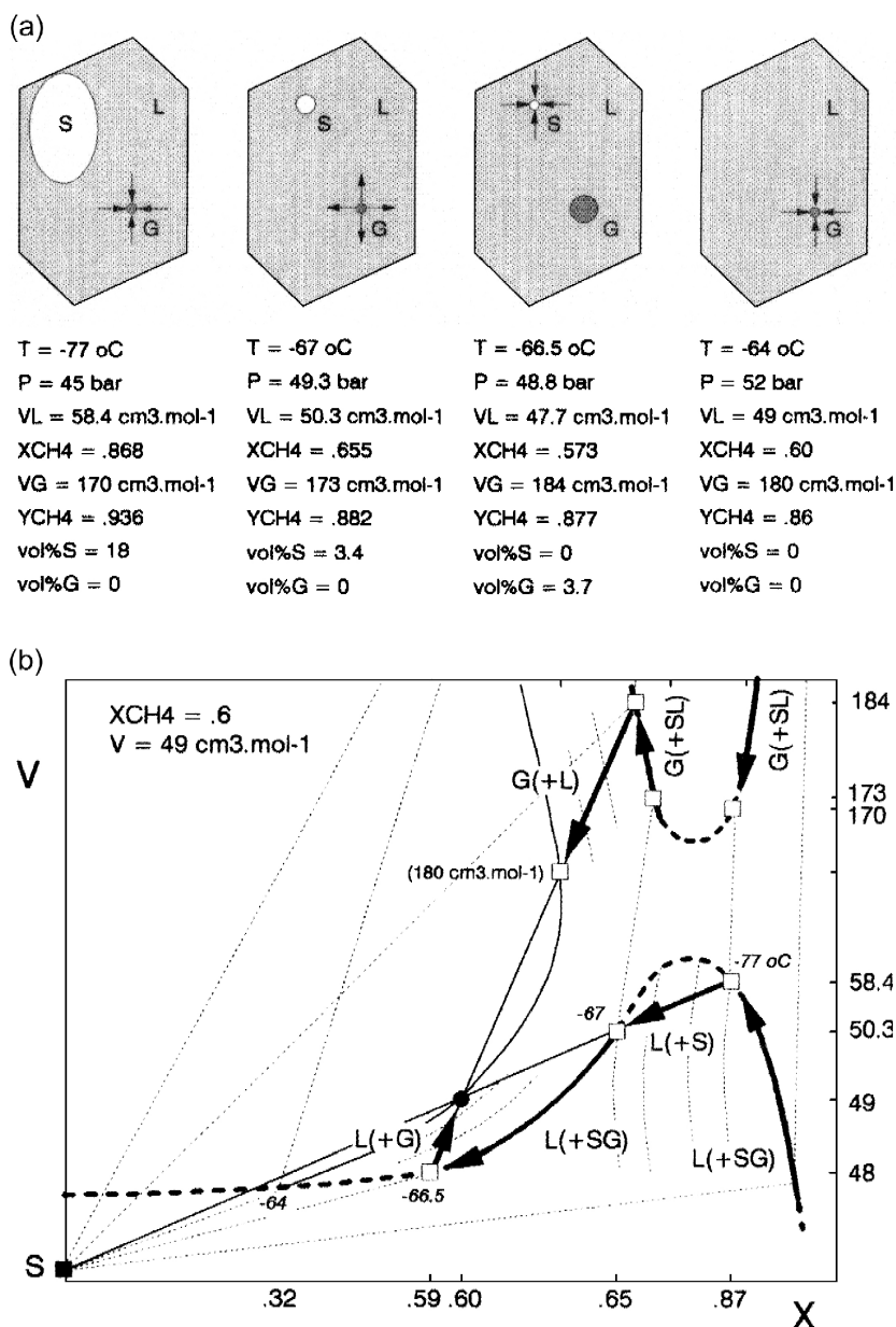
Fig. 11. The molar volume and composition of single phases in \text{CO}_2\text{--CH}_4 fluid inclusion with bulk properties of X_{\text{CH}_4} = 0.60 and V = 49 \text{ cm}^3/\text{mole} showing the phase sequence \text{SLG} \rightarrow \text{SL} \rightarrow \text{SLG} \rightarrow \text{LG} \rightarrow \text{L} (see text for explanation).
