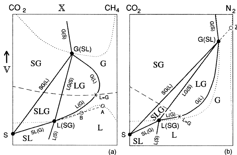
Fig. 7. The topology of isothermal VX diagrams for the systems (a) \text{CO}_2 – \text{CH}_4 and (b) \text{CO}_2 – \text{N}_2 . Stippled curves present the loci of the univariant (polythermal) SLG equilibria for the liquid and gas phases. The dashed lines are the critical curves ( L = G ). Solid lines delimit the phase fields. The SL(G)-curves for different temperatures may in part coincide and represent both partial homogenization, initial melting or bubble nucleation for the same fluid inclusion: e.g. for \text{CO}_2 – \text{CH}_4 the tie-line S–A represents coexisting solid and liquid at the transition SLG → SL (partial homogenization), tie-line S–B at the transition SL → SLG (bubble nucleation), and tie-line S–L(SG) at the transition SLG → LG (final melting). Equally for the system \text{CO}_2 – \text{N}_2 the tie-line S–Z represents the properties of solid and gas at the transition SLG → SL or SLG → SG (partial homogenization), the tie-line S–G(SL) the same properties at the transition SG → SLG (initial melting).
